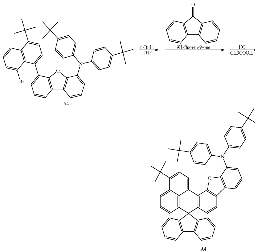
[Reaction Formula 4-2]
