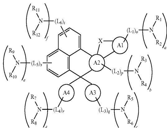
Chemical Formula 1
