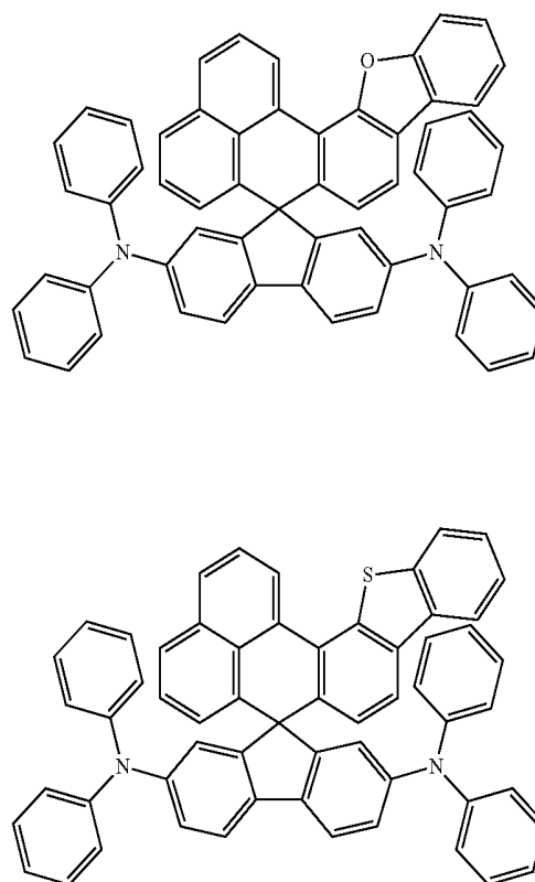
Chemical Formula 4
