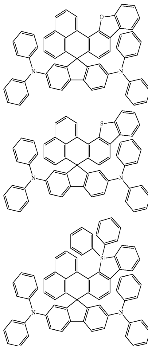
Chemical Formula 4
