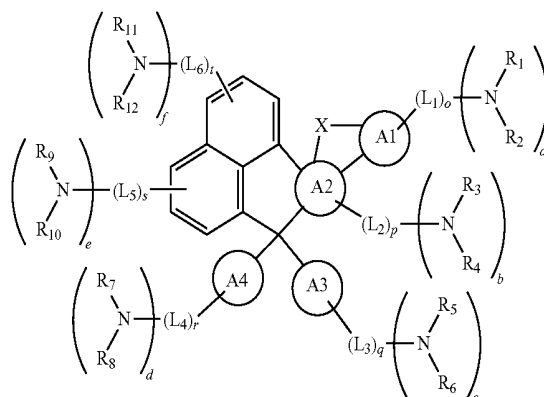
Chemical Formula 1
