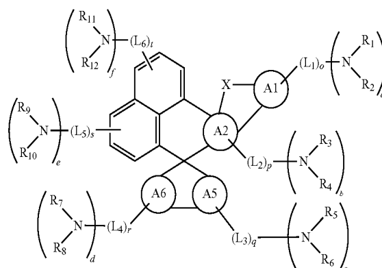
Chemical Formula 3
