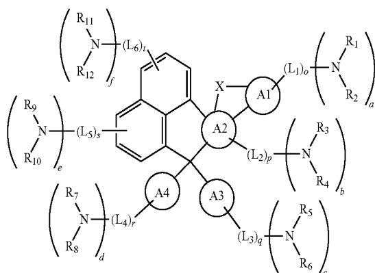
Chemical Formula 1
