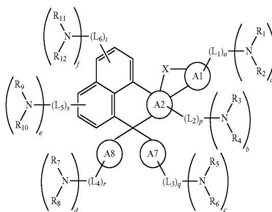
Chemical Formula 3
