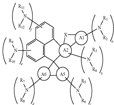
Chemical Formula 5
