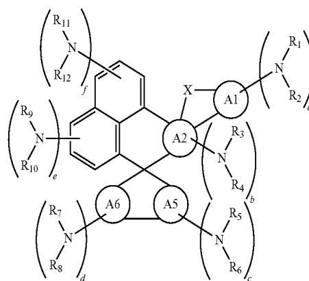
Chemical Formula 5
