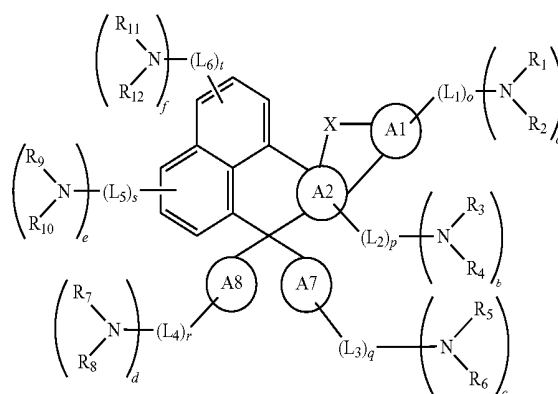
Chemical Formula 3
