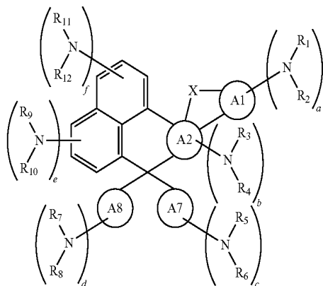
Chemical Formula 6
