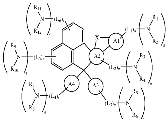
Chemical Formula 1
