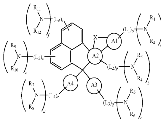
Chemical Formula 1
