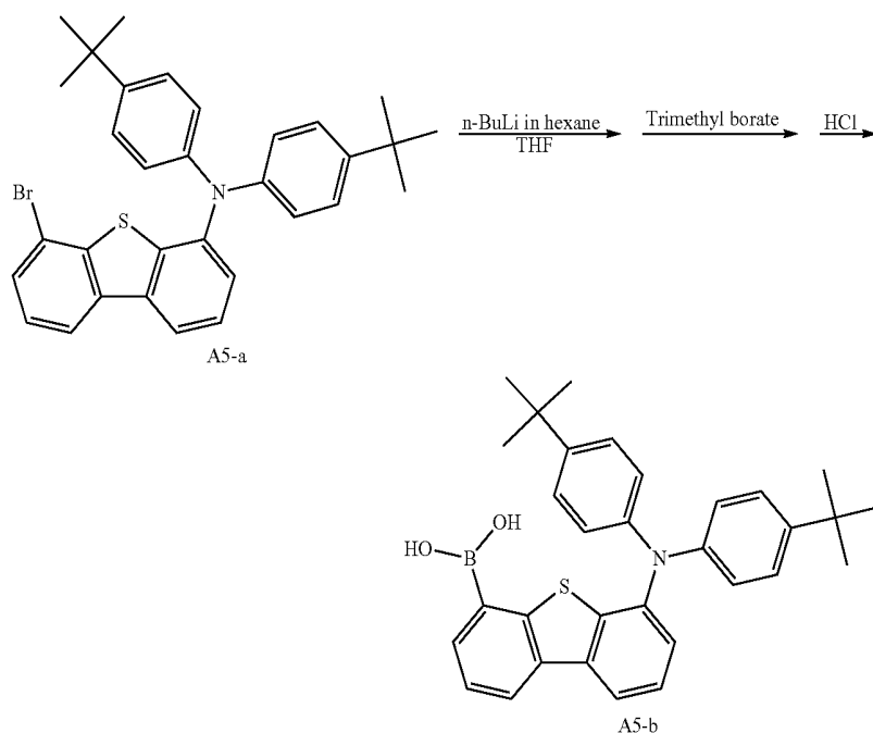
[Reaction Formula 5-2]
